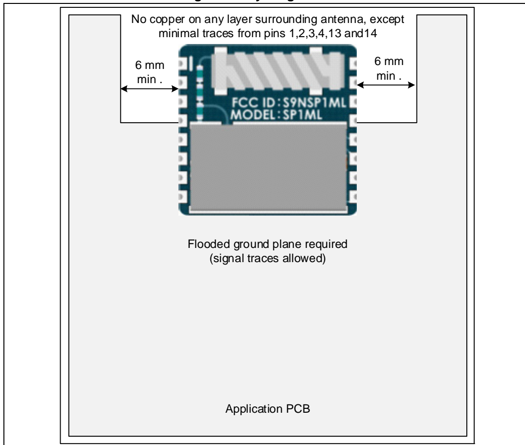
Figure 4. Layout guidelines
