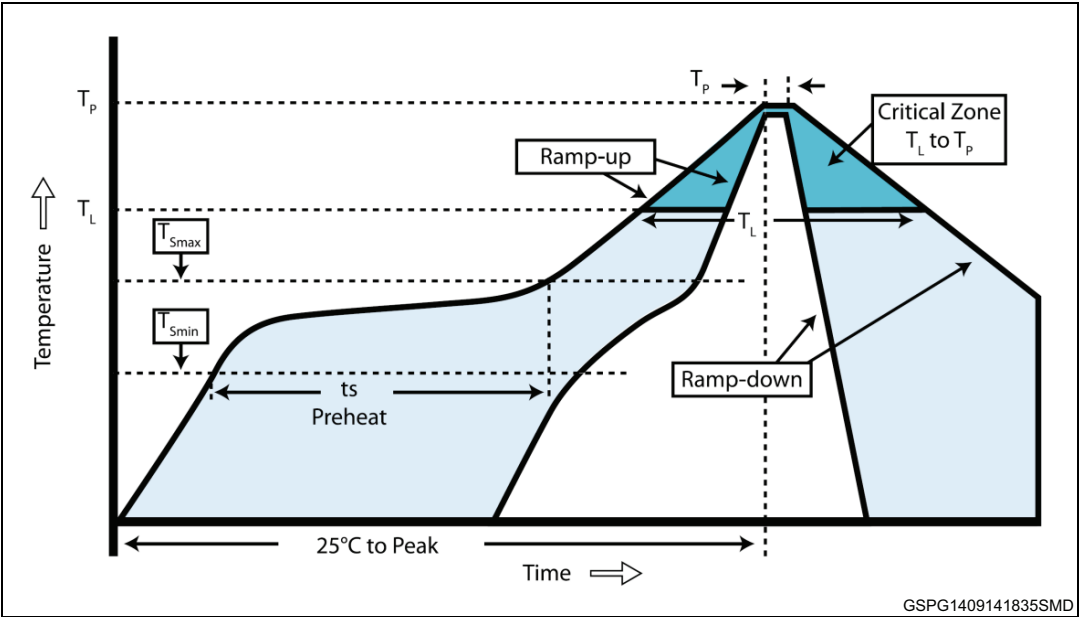
Figure 6. Soldering profile
