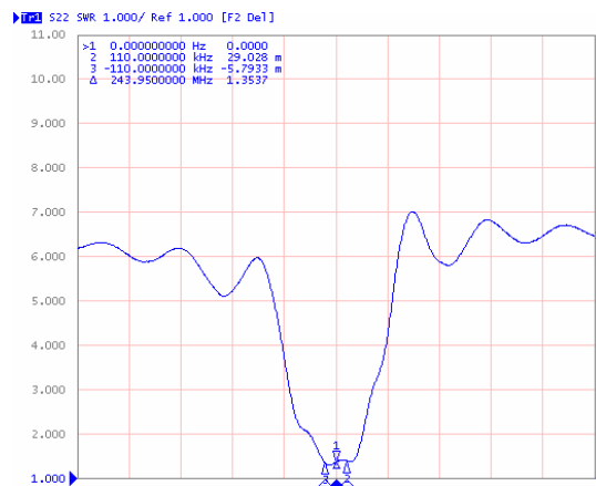
VSWR S22
