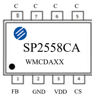
SOP-8
