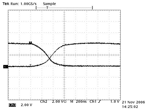
Driver Output Waveform High to Low (SP3083-SP3085)
