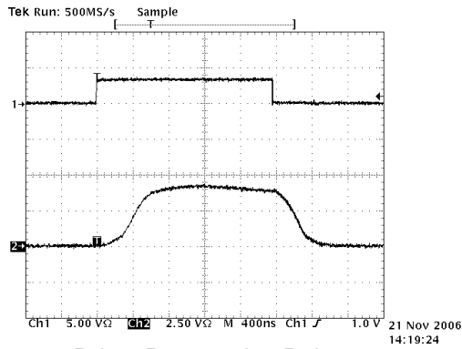
Driver Propagation Delay (SP3083-SP3085)
