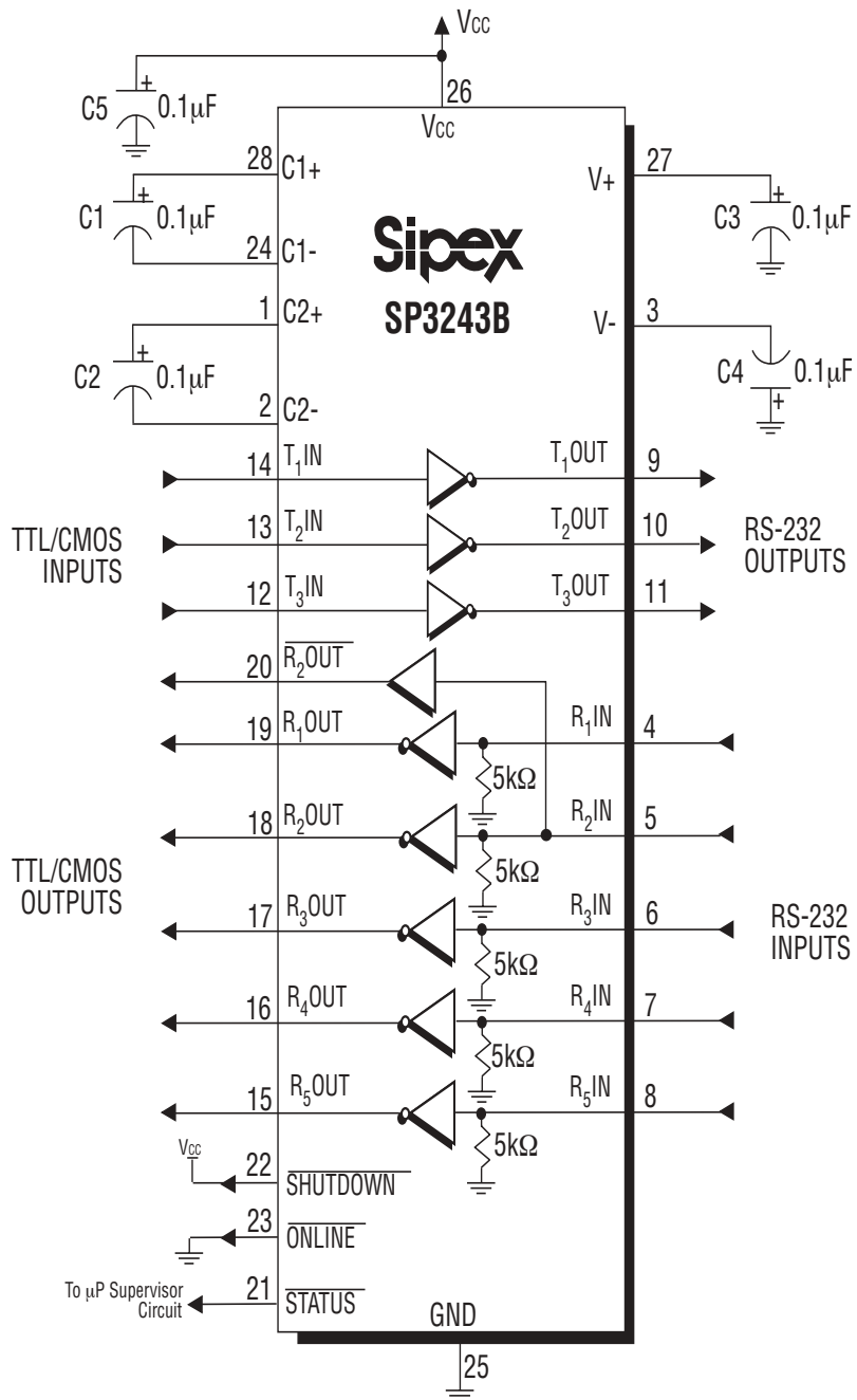
Figure 15. SP3243B Typical Operating Circuit
