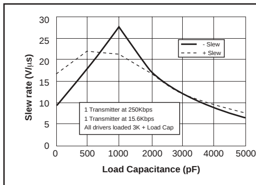
Figure 2. Slew Rate VS. Load Capacitance for the SP3223B
