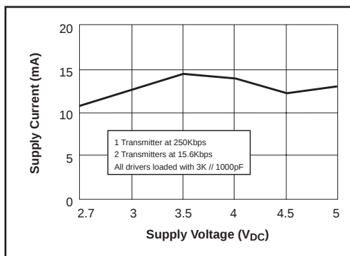
Figure 4. Supply Current VS. Supply Voltage for the SP3243B
