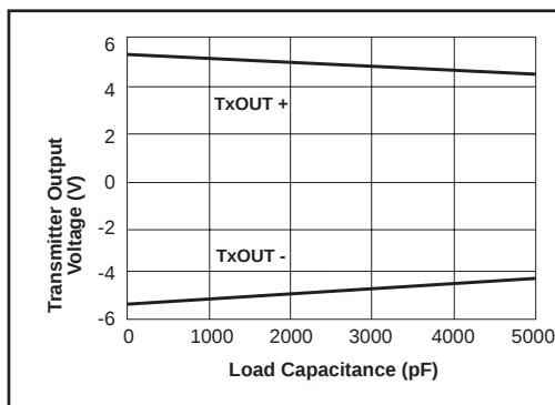
Figure 6. Transmitter Output Voltage VS. Load Capacitance for the SP3243B
