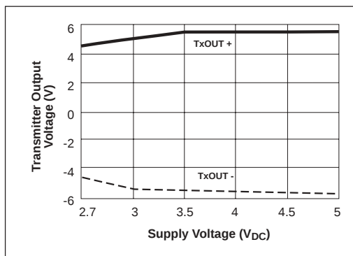
Figure 10. Transmitter Output Voltage VS. Supply Voltage for the SP3243B
