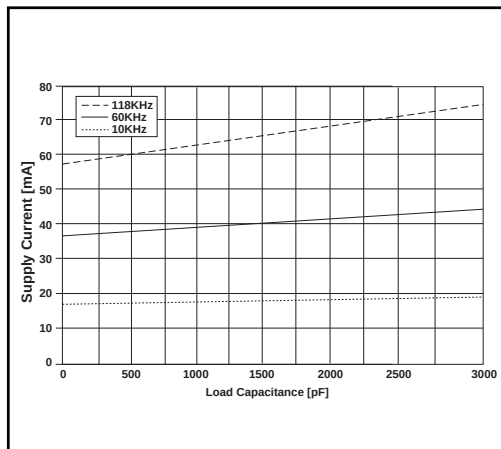
Figure 6. Supply Current VS. Load Capacitance when Transmitting Data for the SP3243H
