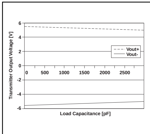
Figure 4. Transmitter Output Voltage VS. Load Capacitance for the SP3243H
