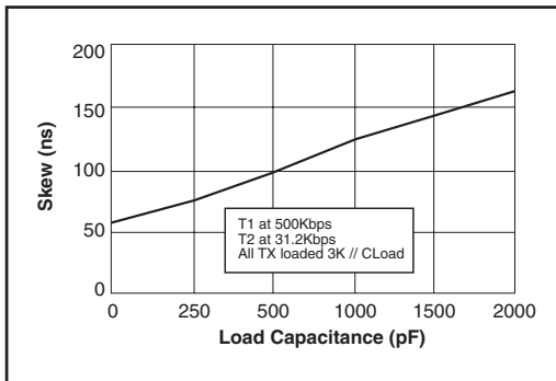
Figure 1. Transmitter Skew VS. Load Capacitance for the SP3223U / SP3243U
