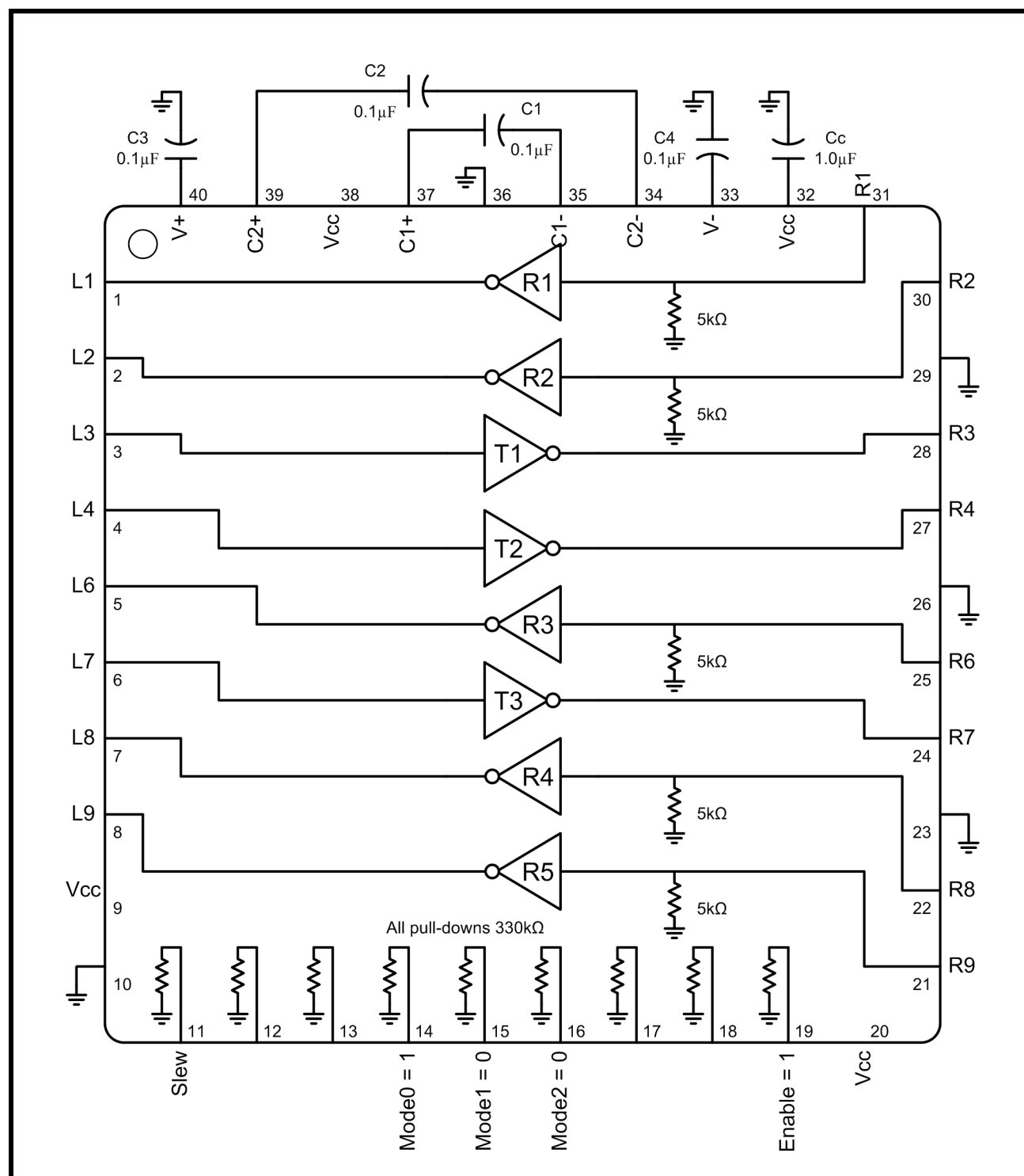
FIGURE 2. MODE 001 - RS-232
