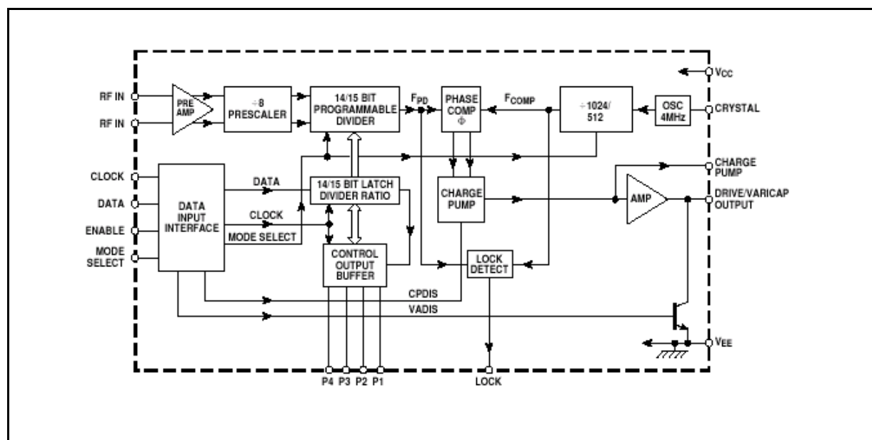
Figure 1 - Block Diagram
