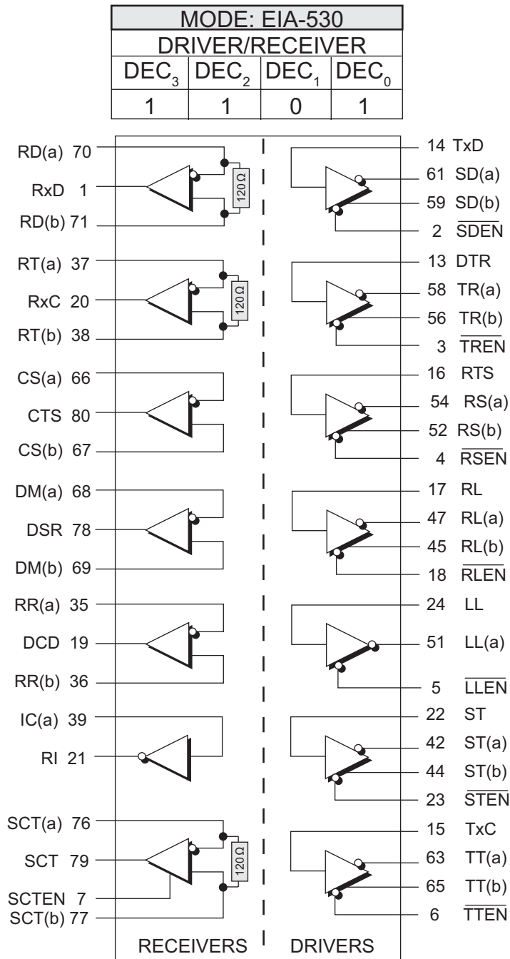
Figure 58. Mode Diagram — EIA-530
