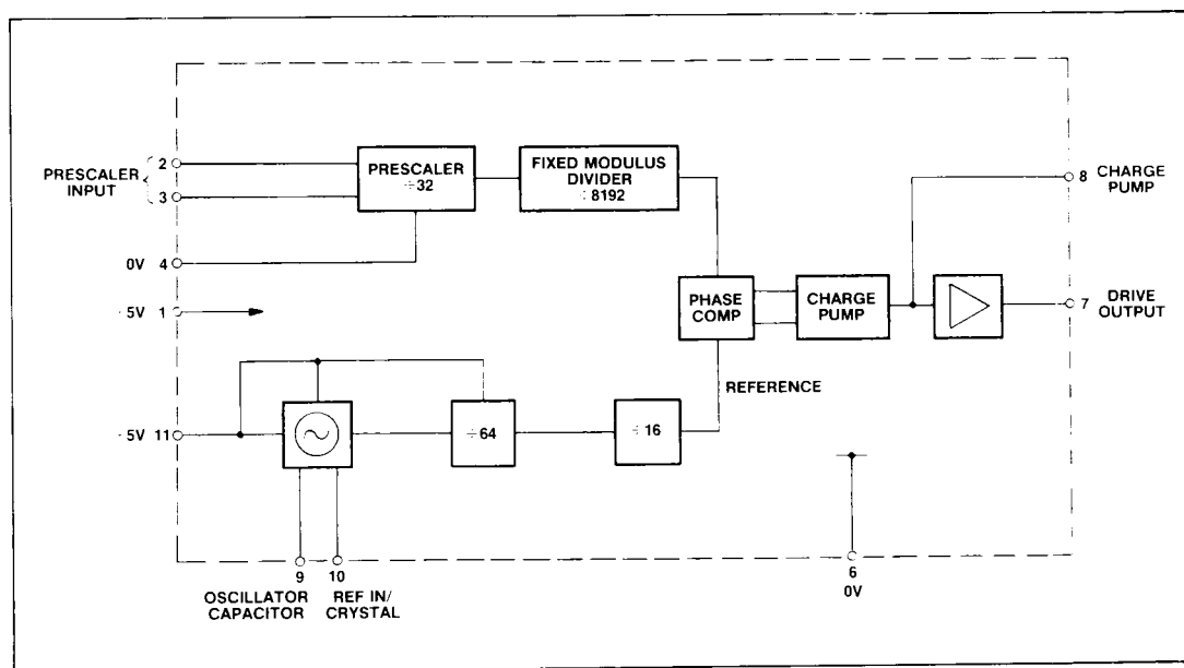
Fig.2 Block diagram
