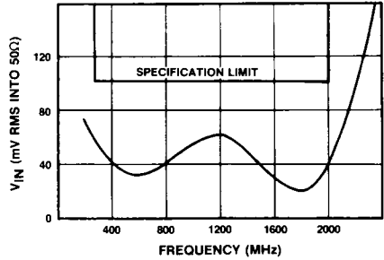
Fig.7 SP5060 typical input sensitivity
