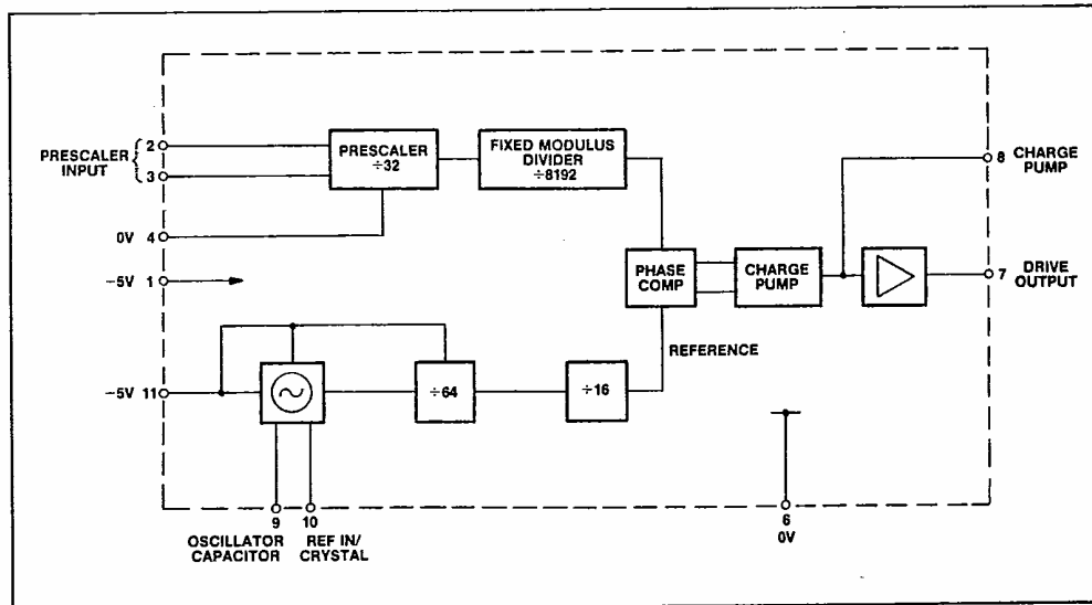
Fig.2 Block diagram
