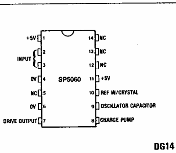
Fig.1 Pin connections - top view
