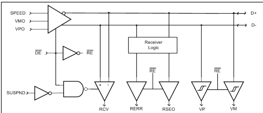
Figure 1. Block Diagram
