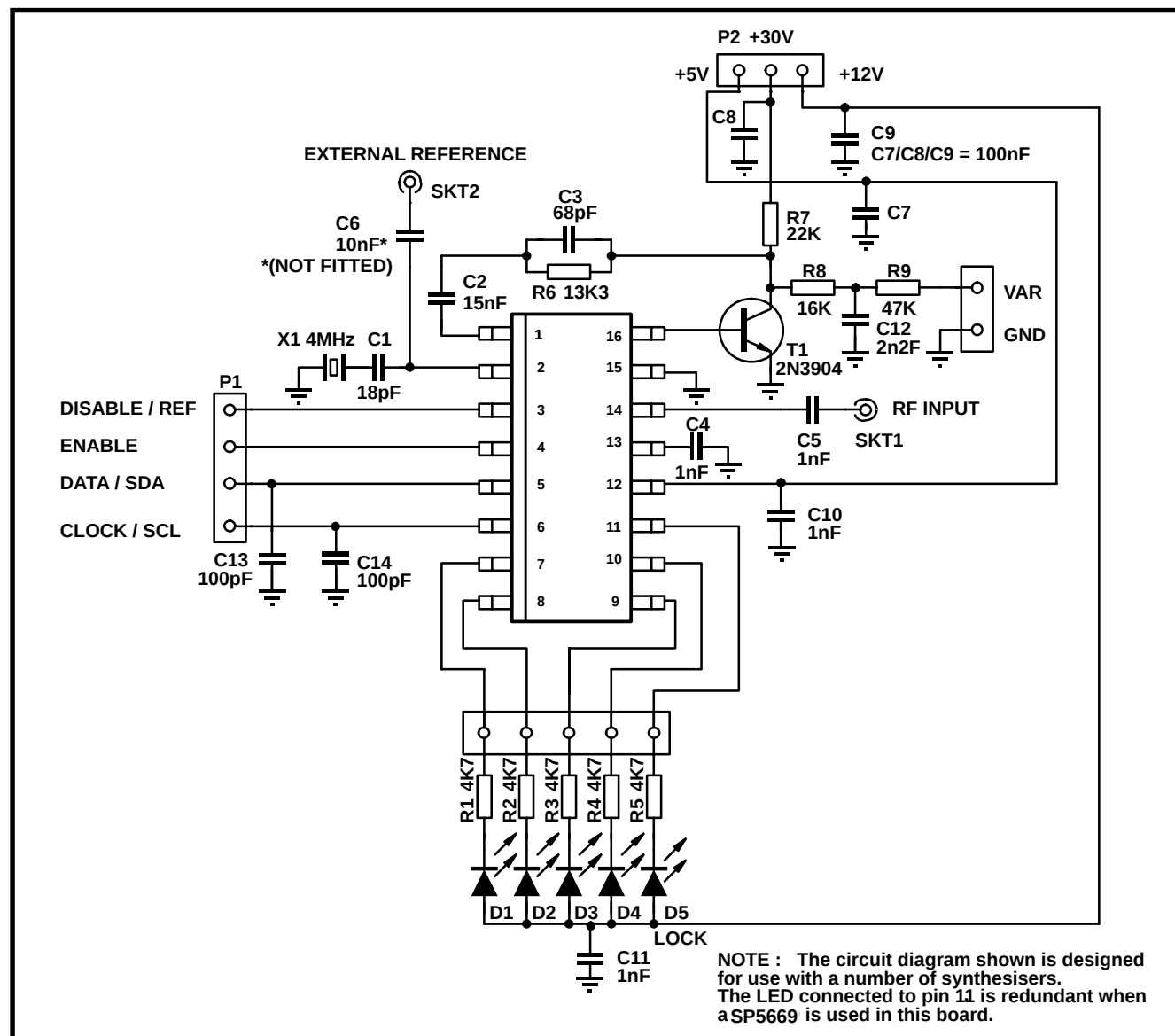
Figure. 10 Test board
