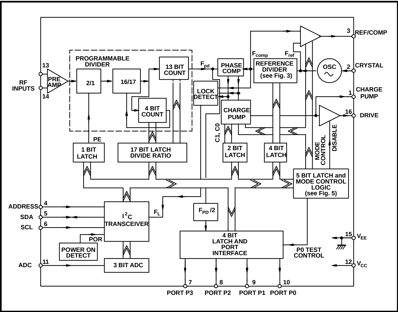
Figure. 2 Block diagram
