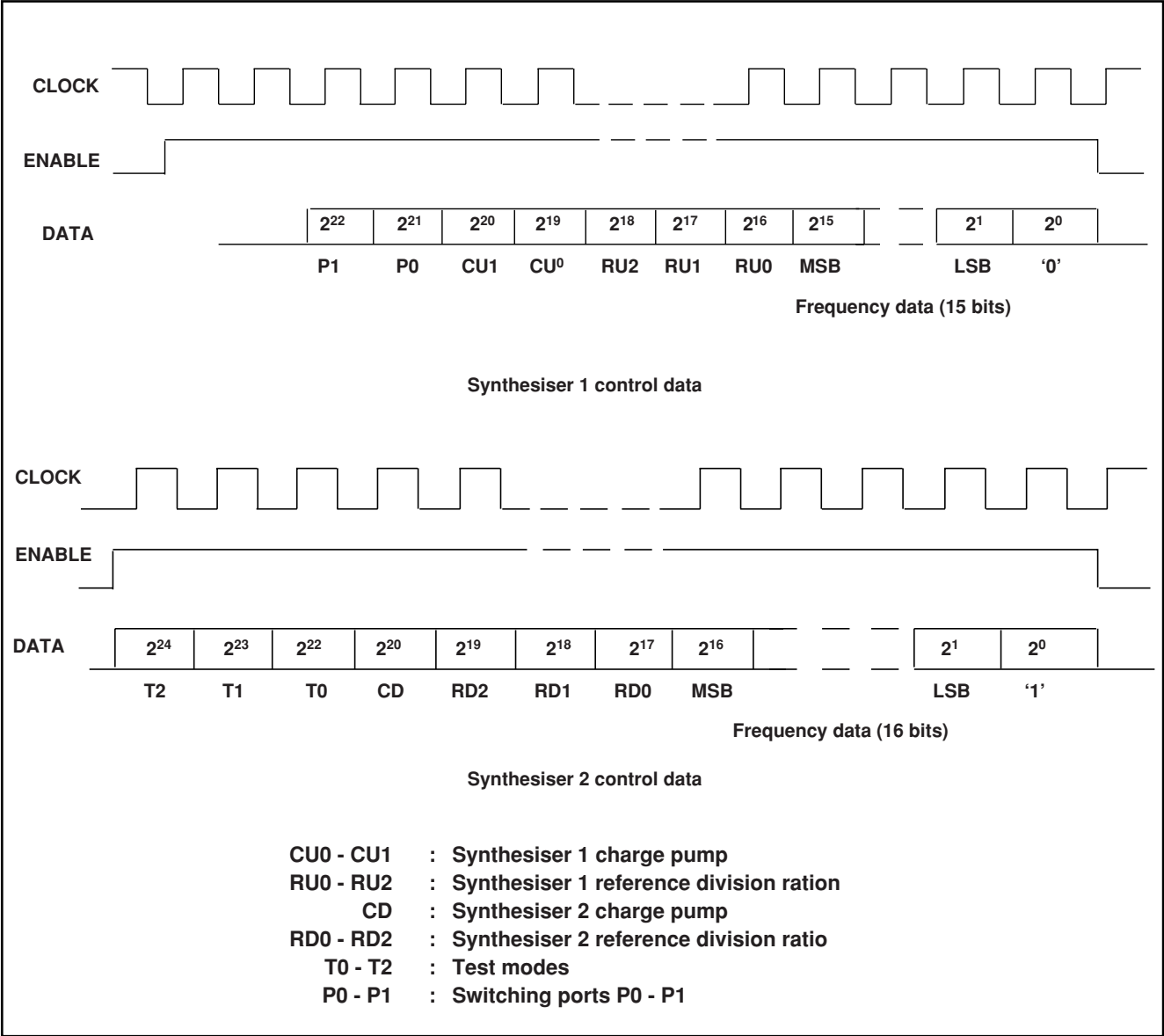
Figure 3 - Control data
