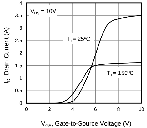
Figure 2. Transfer Characteristics
