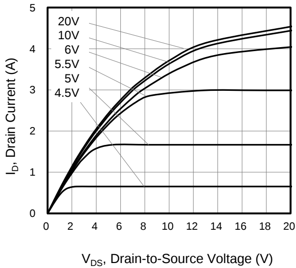
Figure 1. Output Characteristics
