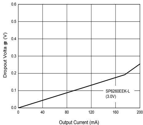
SP6260EEK-L (3.0V) Dropout Voltage vs. Output Current
