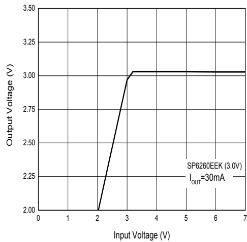
Output Voltage vs. Input Voltage SP6260EEK (3.0V)
