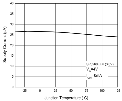
Supply Current vs. Junction Temperature SP6260EEK (3.0V)
