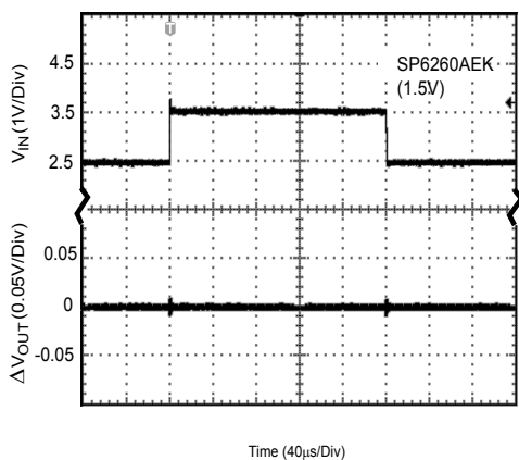
SP6260AEK (1.5V) Line Transient (Conditions: I_{OUT}=30mA , C_{IN}=1\mu F , C_{OUT}=1\mu F )
