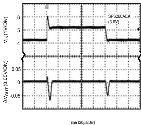
SP6260EEK (3.0V) Line Transient (Conditions: I_{OUT}=30mA , C_{IN}=1\mu F , C_{OUT}=1\mu F )
