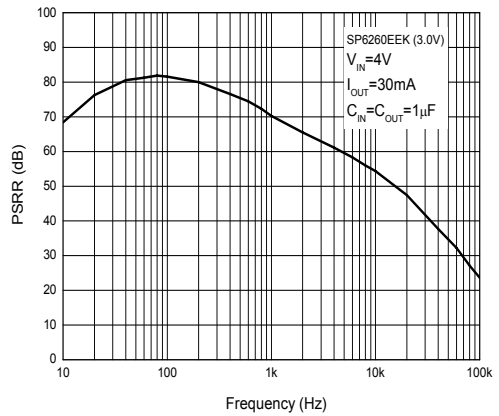
PSRR vs. Frequency SP6260EEK (3.0V)
