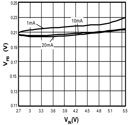
Feedback Voltage vs. V_{IN} (4LEDs)
