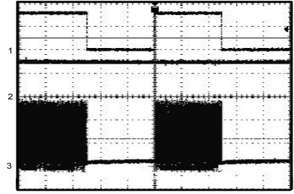
Start-Up/Shutdown
