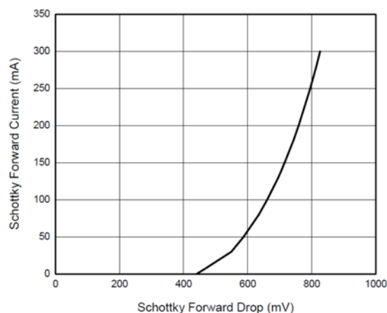
Fig. 7: Schottky Forward Current vs Schottky Forward Drop
