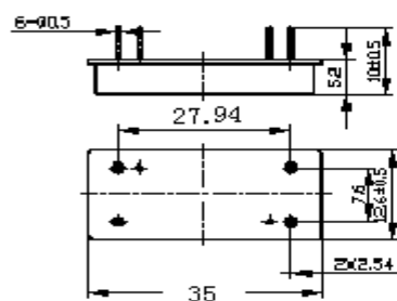
Package Outline
