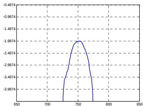
Passband Response
