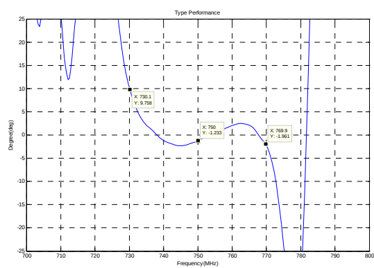
Phase Linearity(f0±20MHz)
