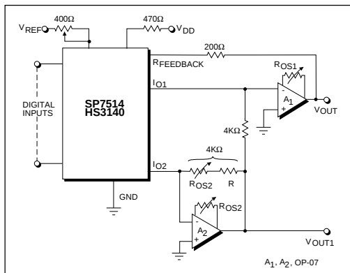
Figure 3. Bipolar Operation
