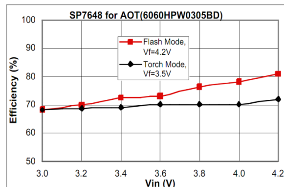
Fig. 9: Efficiency versus Input Voltage
