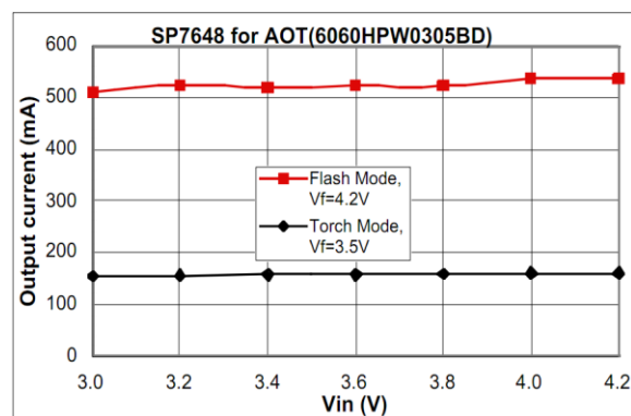
Fig. 8: Output Current versus Input Voltage
