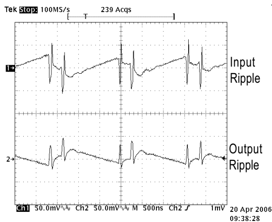
Ripple 1X Torch 200mA, V_{IN}=4.2V
