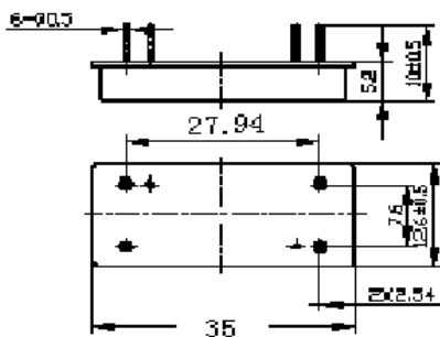
Package Outline
