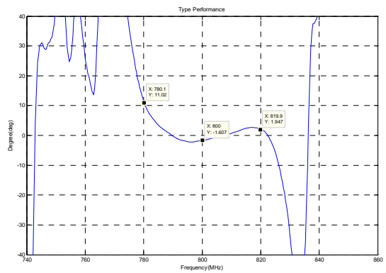
Phase Linearity(f0±20MHz)
