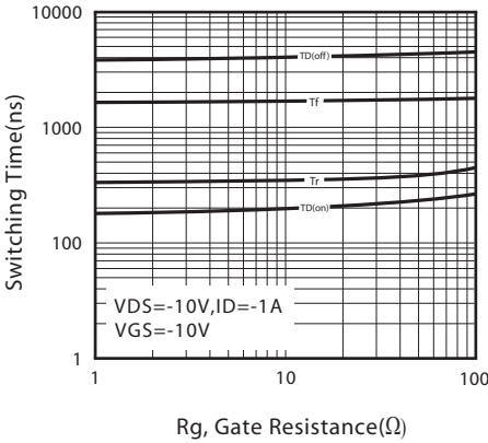
Figure 10. switching characteristics
