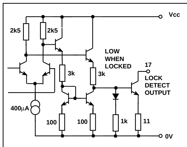
Fig. 7d Lock detect output
