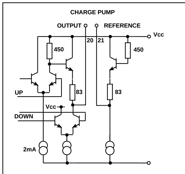
Fig. 7f Charge pump circuit
