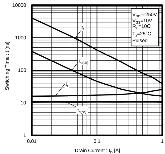
Fig.10 Switching Characteristics
