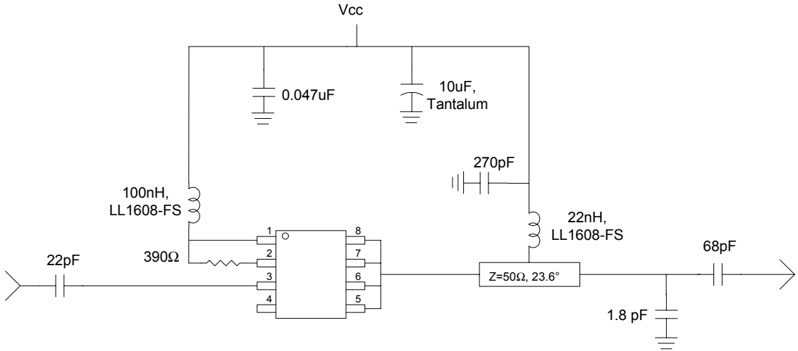
1930-1990 MHz Schematic
