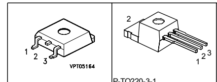
P-TO263-3-2
