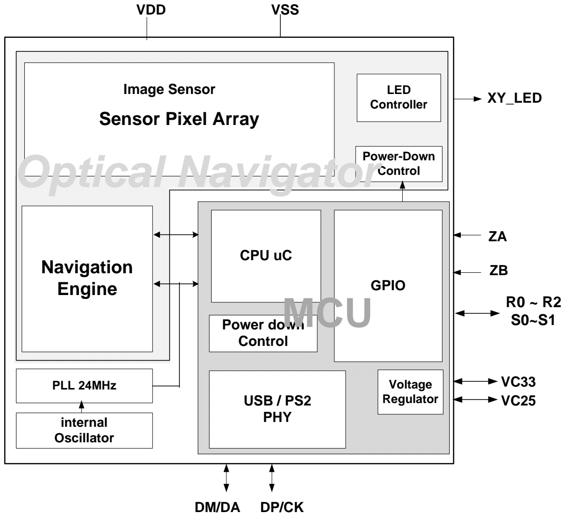
Figure 9: Block Diagram
