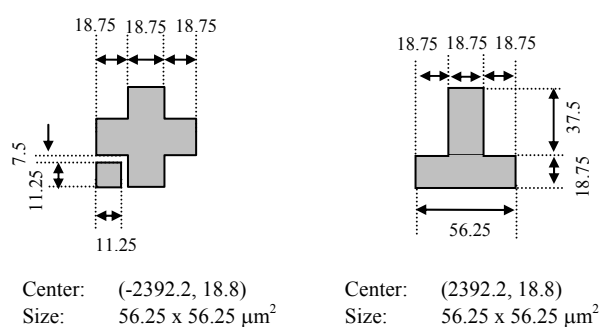
Figure 5-2: SPD0301Z alignment mark dimension
