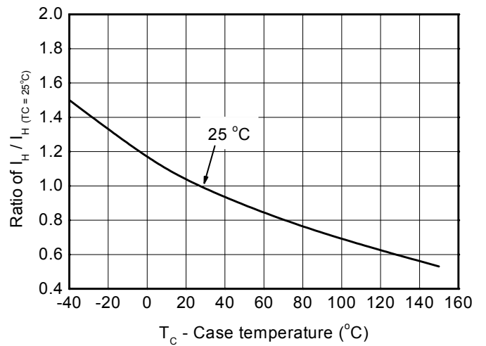
Normalized holding current vs. Case temperature
