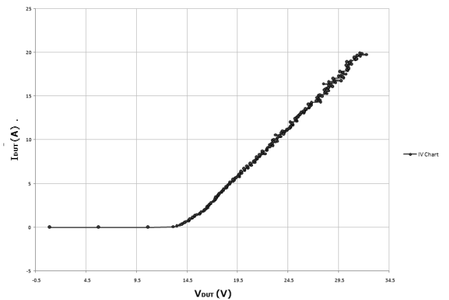
TLP test
