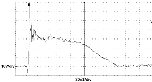
ESD Clamping Voltage (IEC61000-4-2 +8kV contact)
