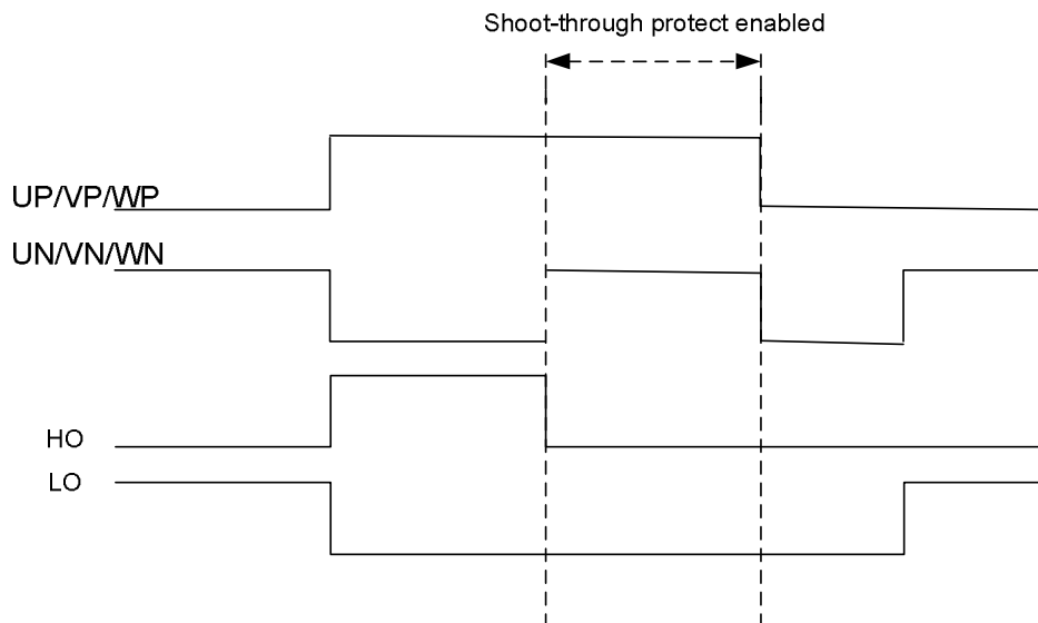
Figure 10 . Shoot-through (cross-conduction) protection
