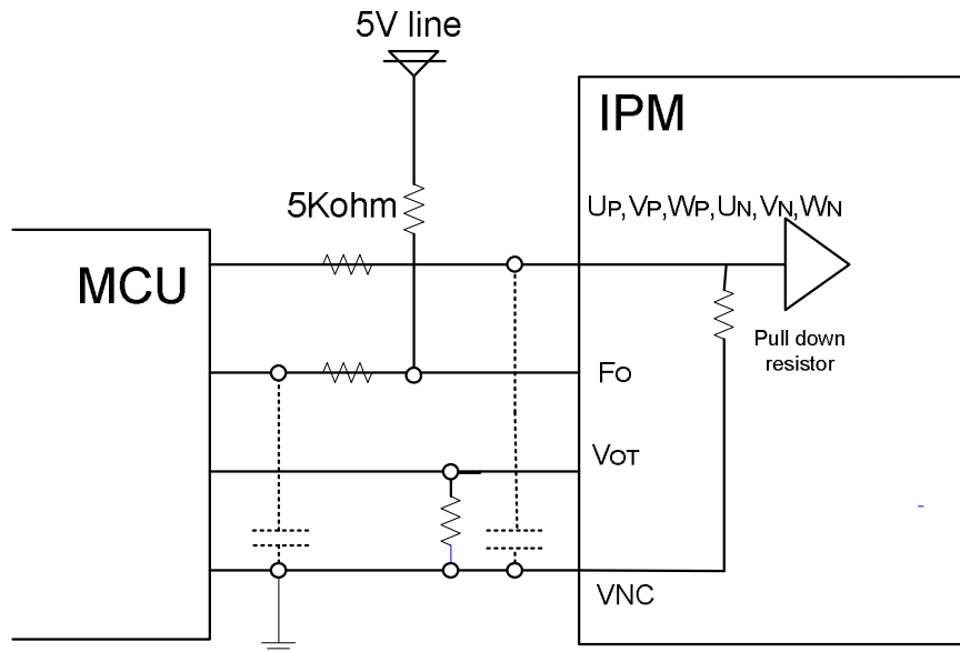
Figure 14. Recommended CPU I/O Interface Circuit
