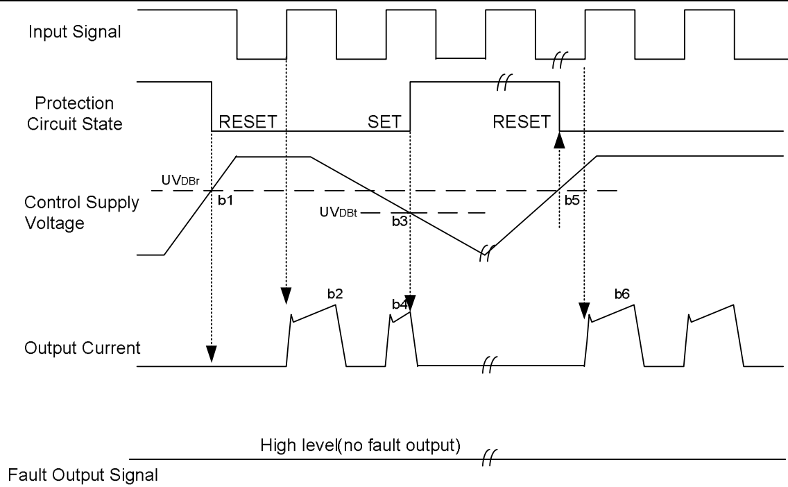
Figure 12. Under-Voltage Protection (High-side Operation only)
