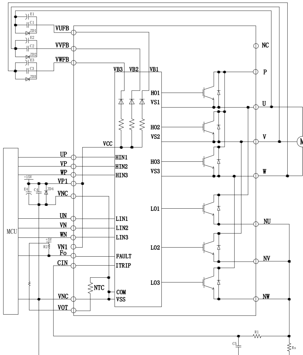
Figure 16. Typical Application Circuit
