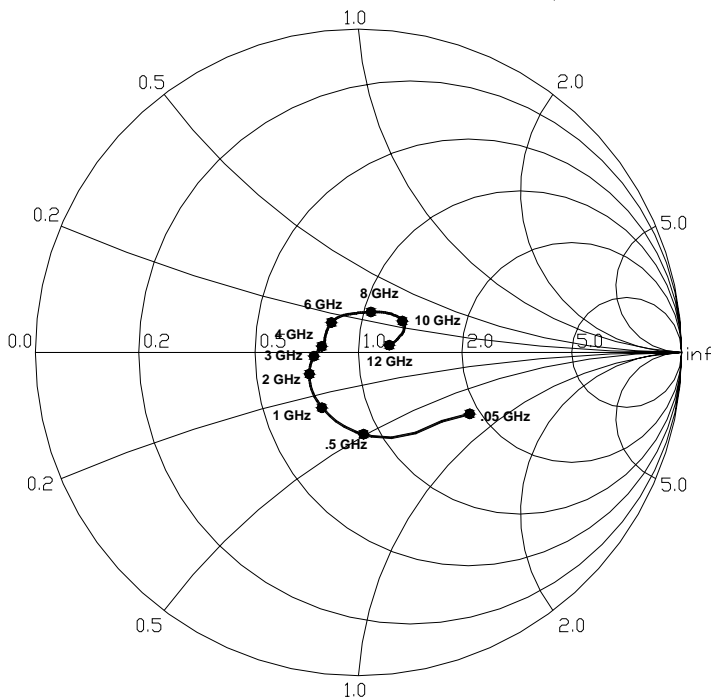
S11 vs. Frequency
