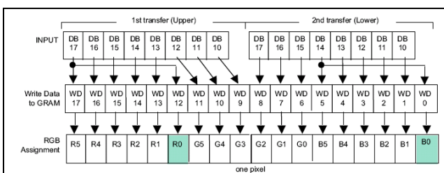
Figure 6-13 8-bit interface (65,536 colors) TRIREG = 0, DFM=x
