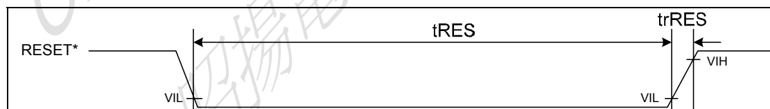
Figure 14-2 Reset Operation
