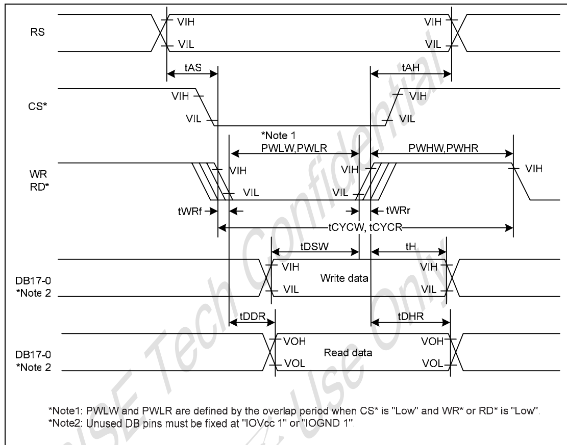
Figure 14-1 80-System Bus Interface
