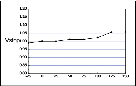
Figure 6. Stop Threshold Voltage
