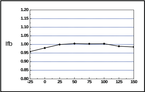
Figure 2. Feedback Source Current
