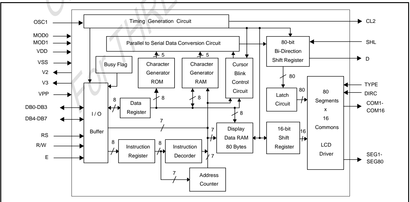
Figure 4-1: Block Diagram
