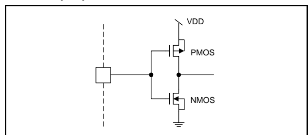
Figure 6-36: Input port: E Configuration
