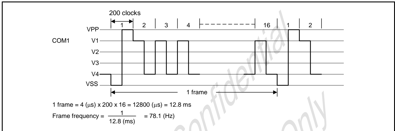
Figure 6-32: 1/16 Duty type-A waveform
