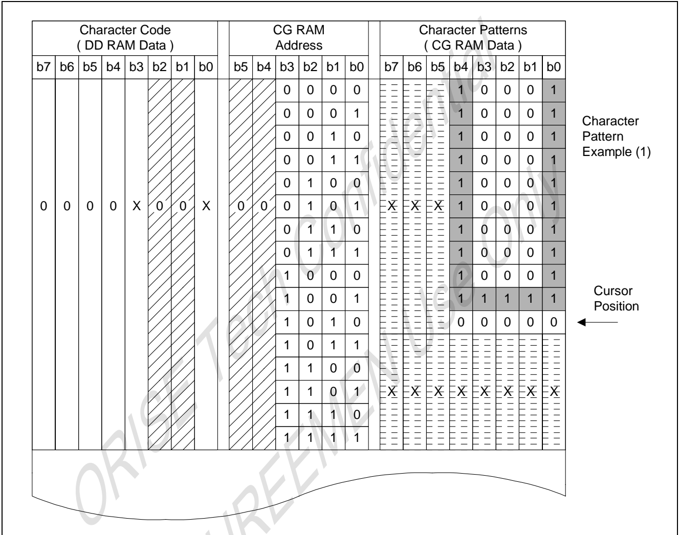
Figure 6-25: 5 x 10 Dot Character Patterns
