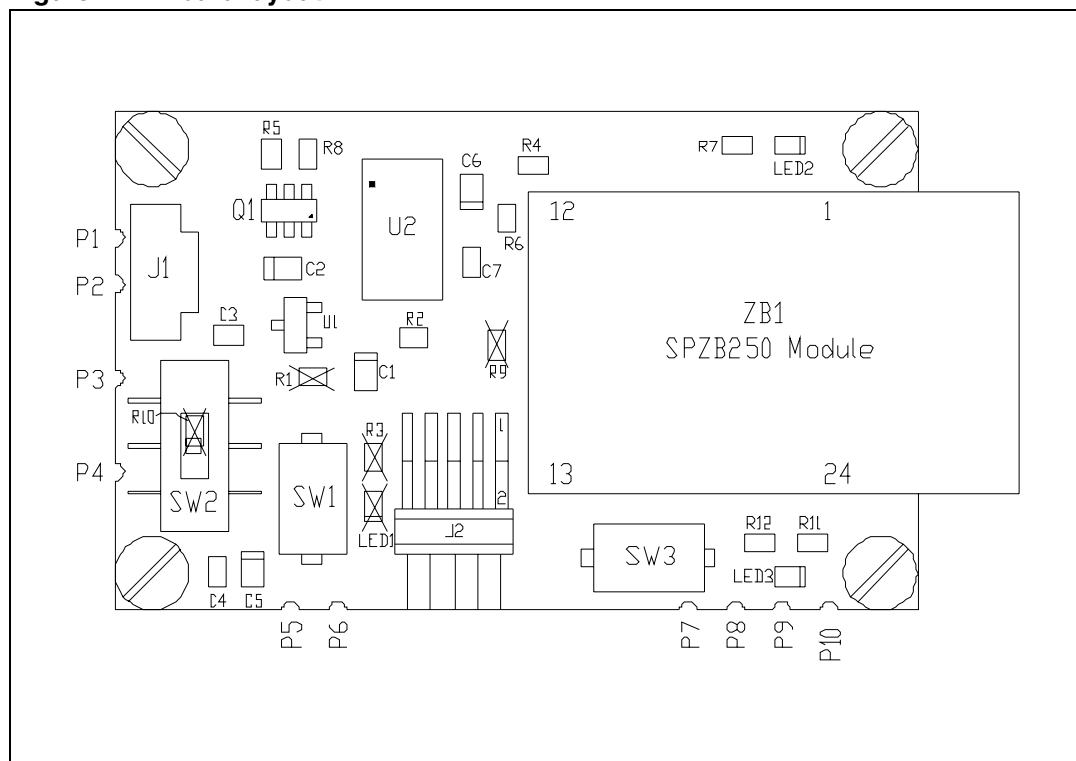
Figure 7. Board layout
