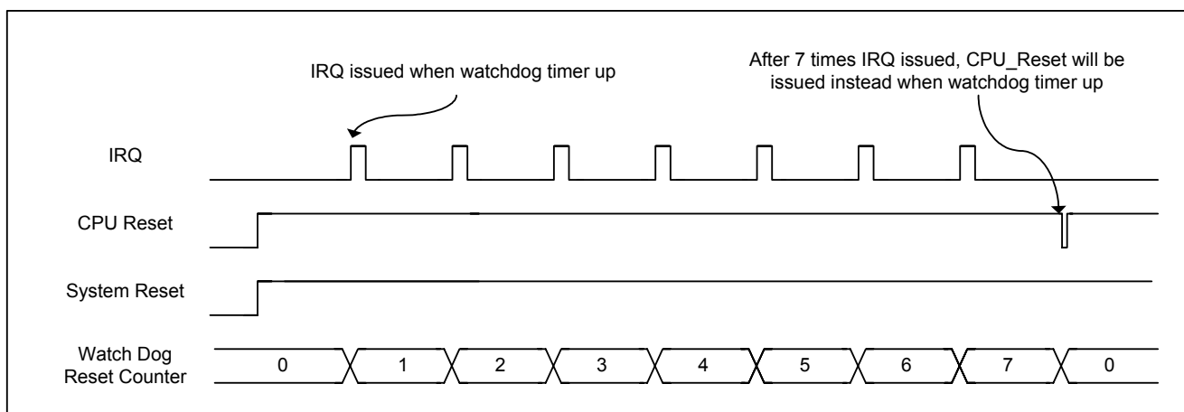
Figure 5.6-5 Watchdog reset sequence
