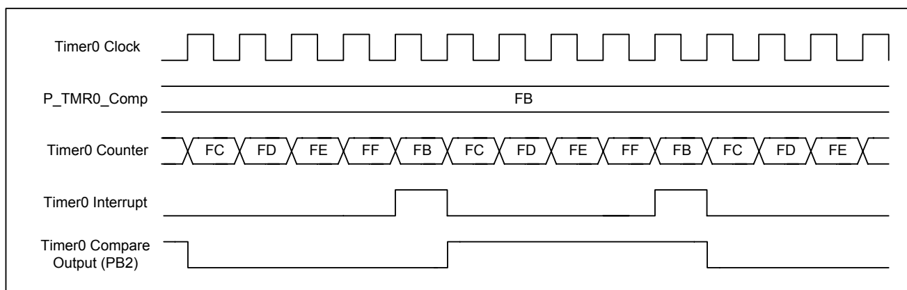
Figure 5.9-1 8-bit compare waveform
