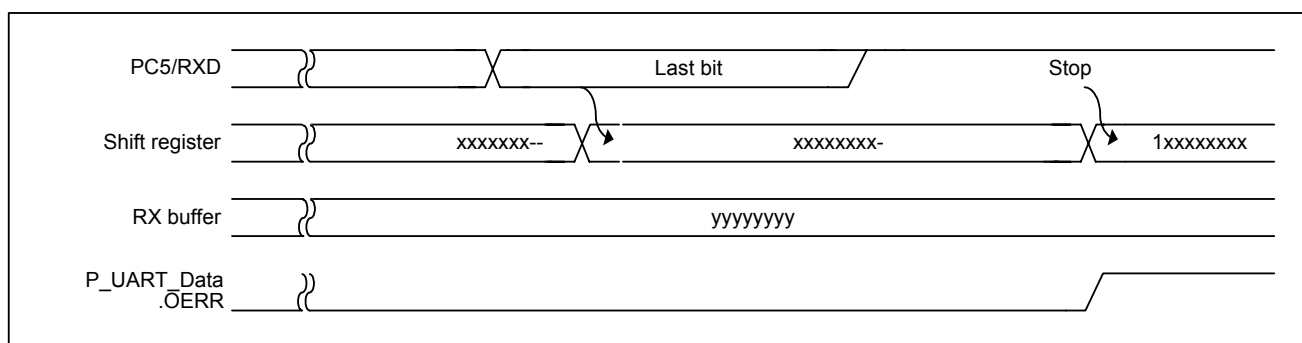
Figure 5.11-8 Overrun error timing
