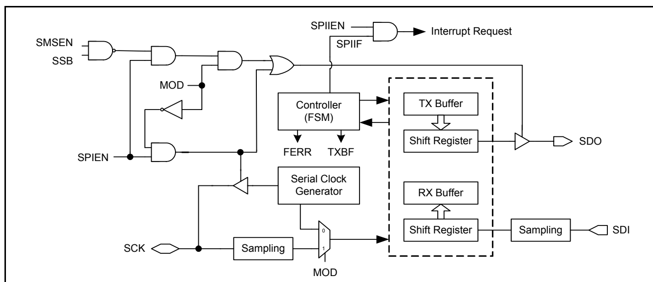
Figure 13.1 SPI structure
