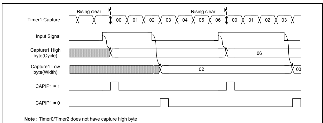
Figure 5.9-3 8-Bit capture waveform
