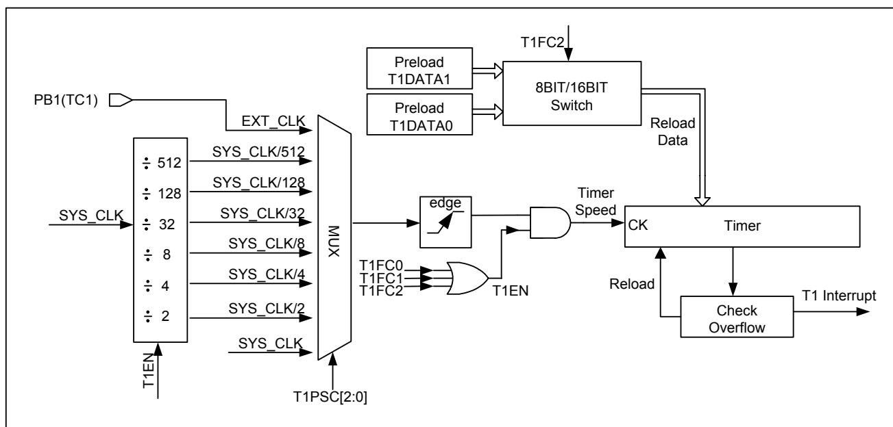
Figure 5.8-4 16-bit timer block diagram
