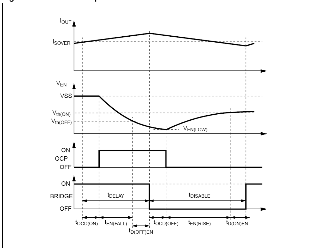
Figure 21. Overcurrent protection waveforms
