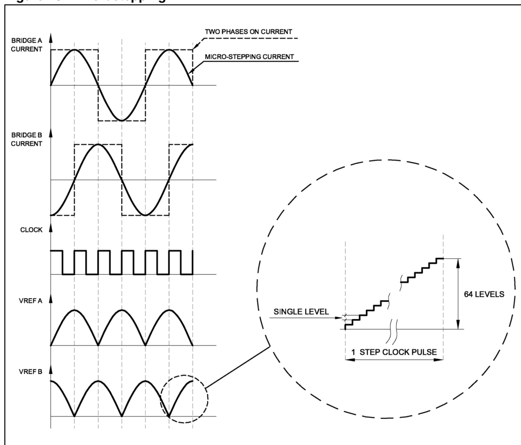
Figure 20. Microstepping
