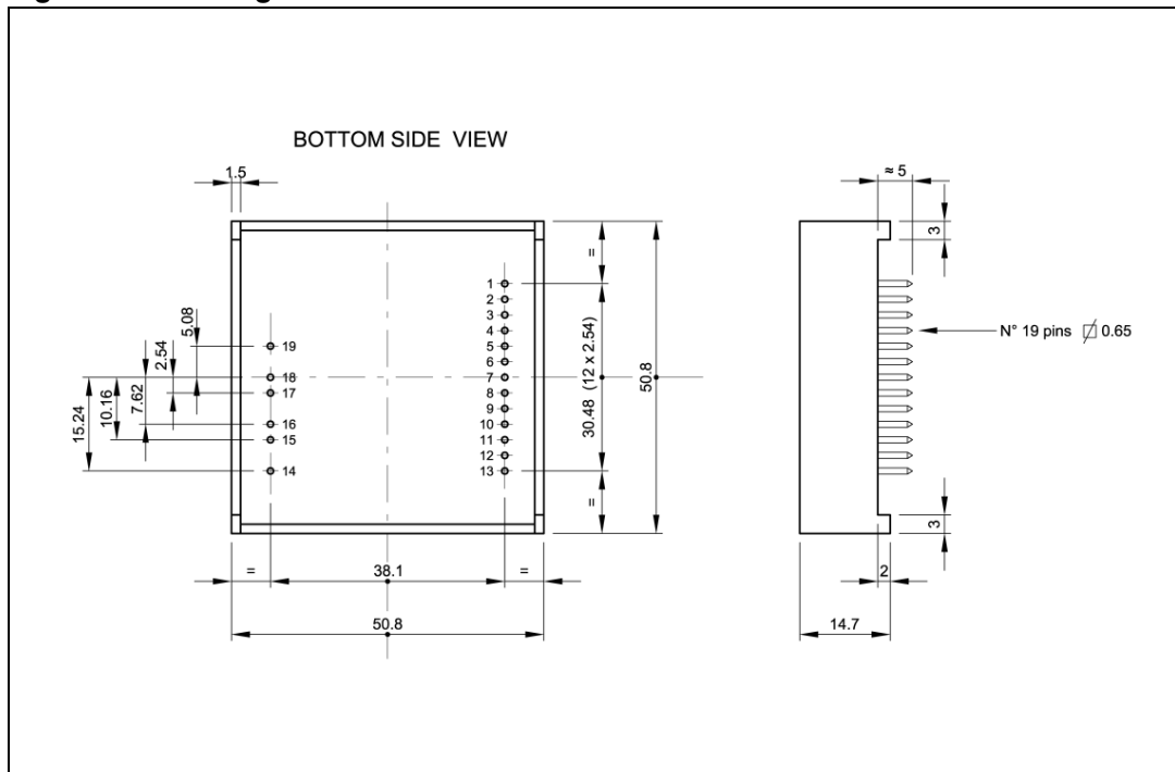
Figure 22. Package dimensions
