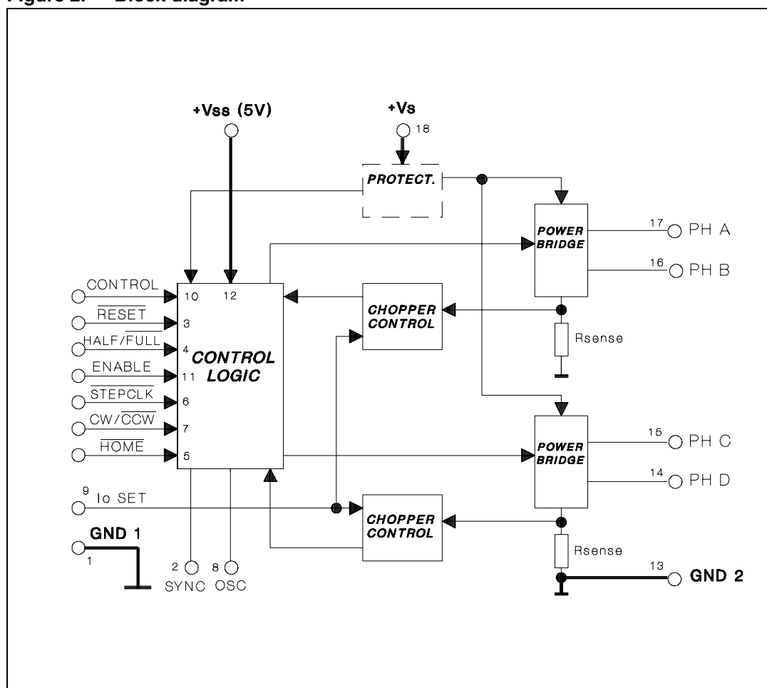
Figure 2. Block diagram
