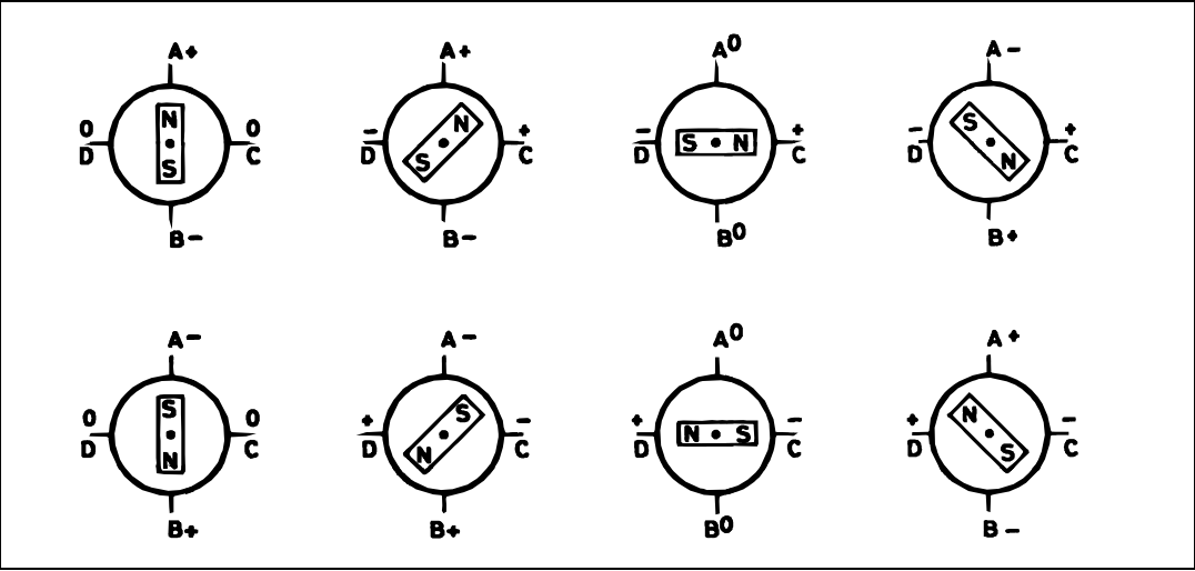
Figure 8. Half step sequence
