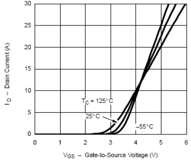
Transfer Characteristics
