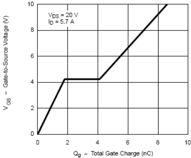
Gate Charge
