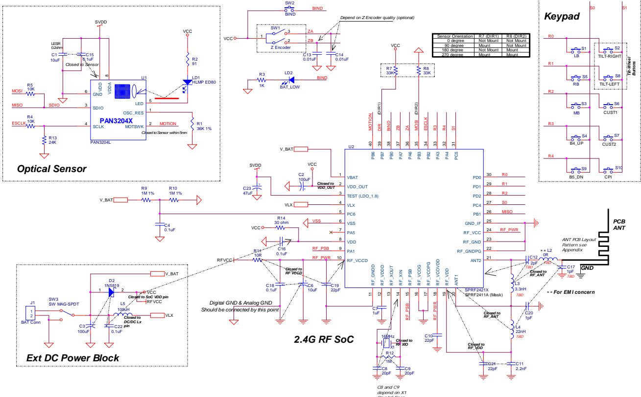
2.4GHz RF Mouse SoC device low-power application circuitry (with PAN3204L)
