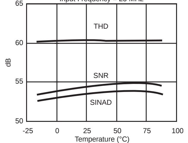
Dynamic Performance vs. Temperature Sample Rate = 80 MSPS Input Frequency = 25 MHz
