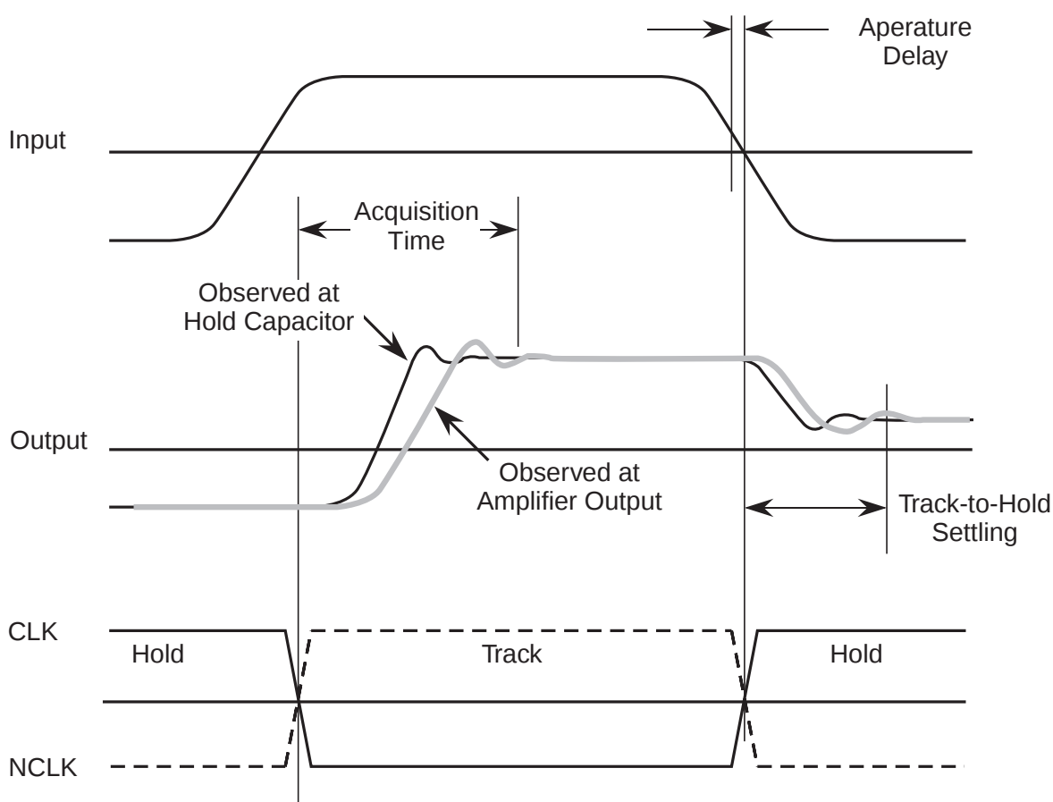
Figure 1 - Timing Diagram
