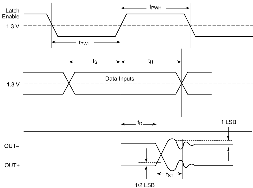
Figure 1 – Timing Diagram
