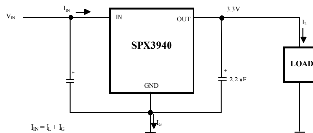
Figure 3. 3.3V Regulator Circuit
